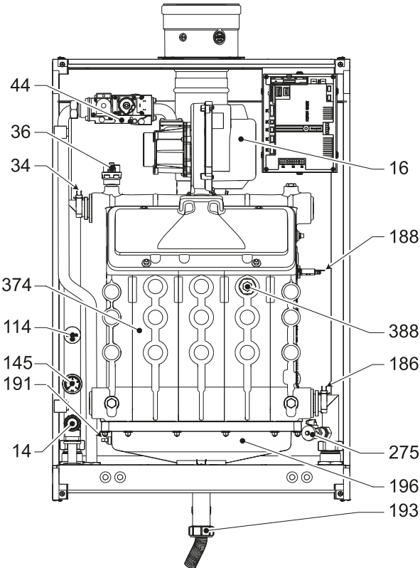
fig. 91- General view - model FORCE W 150
