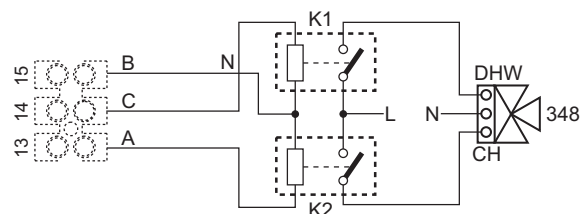
fig. 97- Connection of the 3-way valve with 3 wires
