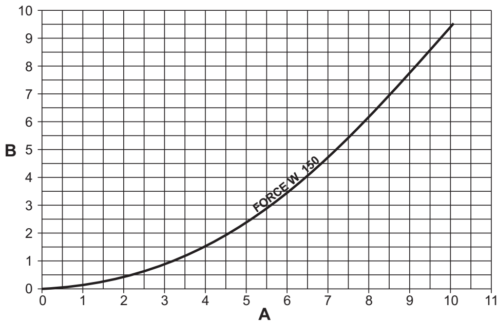
fig. 94- Pressure loss diagram - models FORCE W 150
