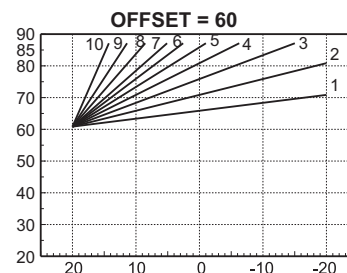
fig. 31- Compensation curve parallel offset
