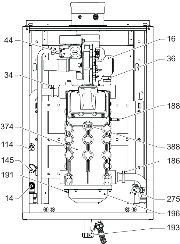
fig. 89- General view - model FORCE W 60 and FORCE W 80
