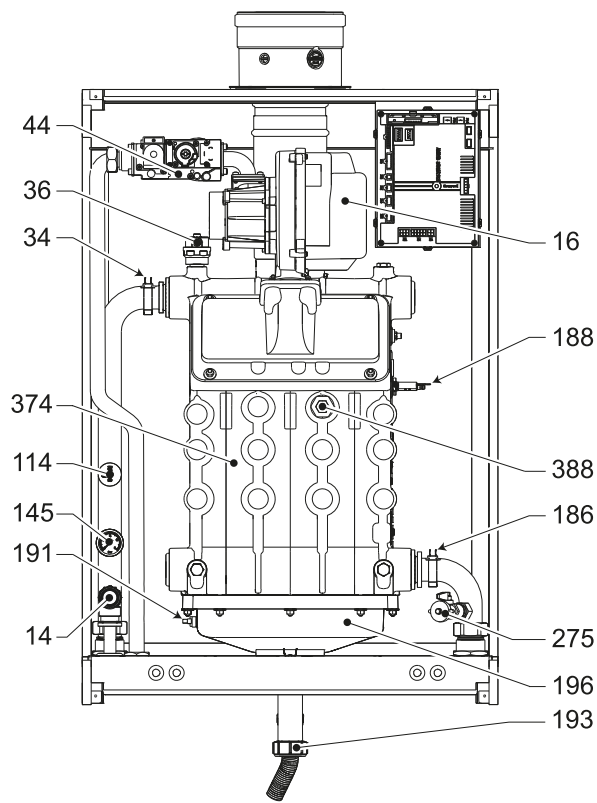
fig. 90- Vista general mods. FORCE W 99 y FORCE W 120
