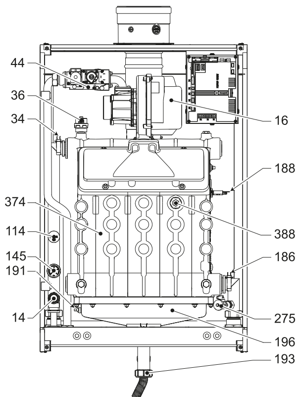
fig. 91- Vista general mod. FORCE W 150
