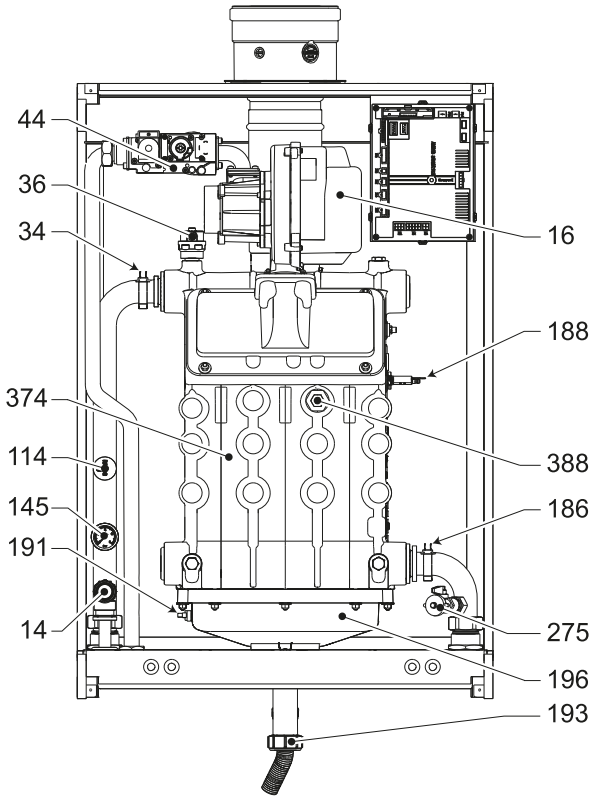
fig. 90- General view - model FORCE W 99 and FORCE W 120
