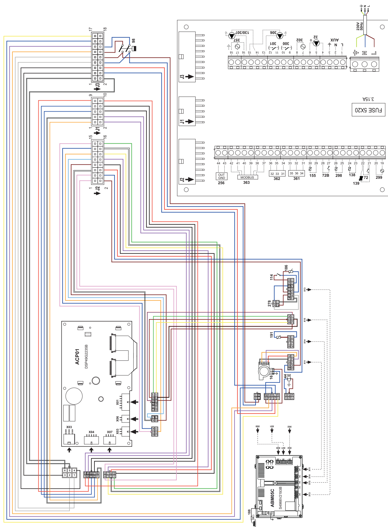
fig. 96- Wiring diagram OPERA 125 and 160
