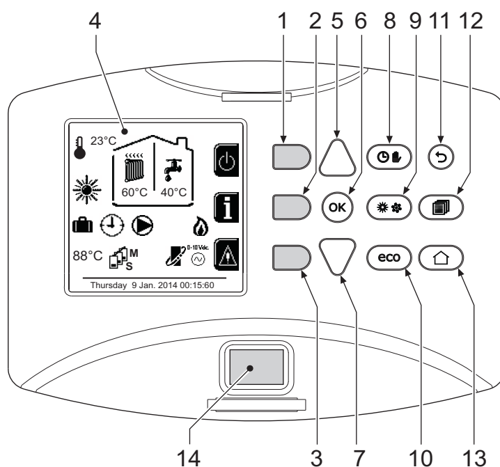
fig. 1 - Control panel
