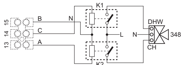
fig. 93- Connection of the 3-way valve with 3 wires
