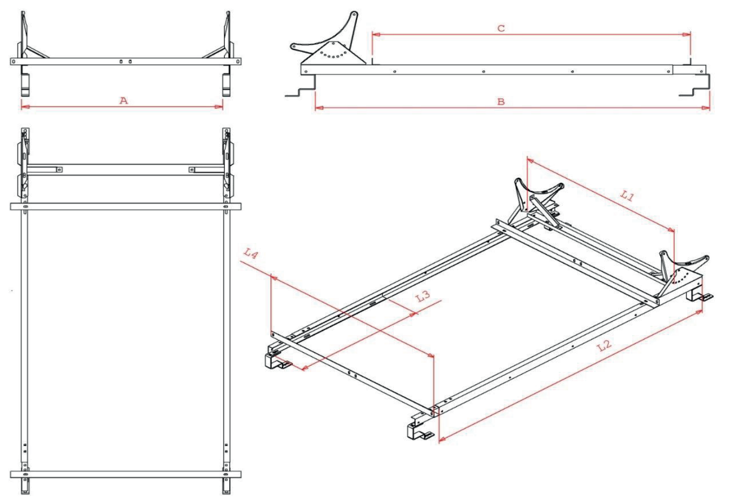
Figure 2: basic installation and system dimensions.
