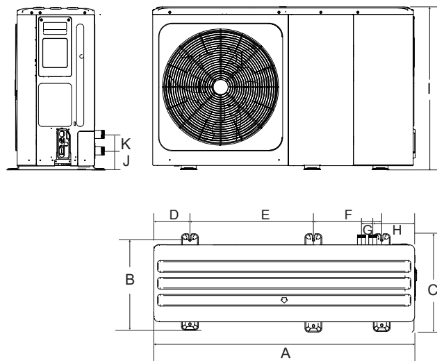
8/10/12/14/16 kW (unitate: mm)
