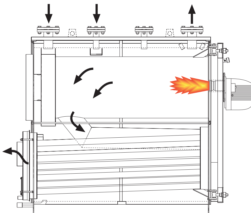
Fig. 1 - Working principle
