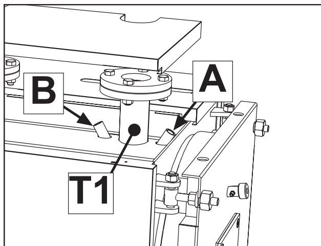
Fig. 15 - Probe and bulb wells
