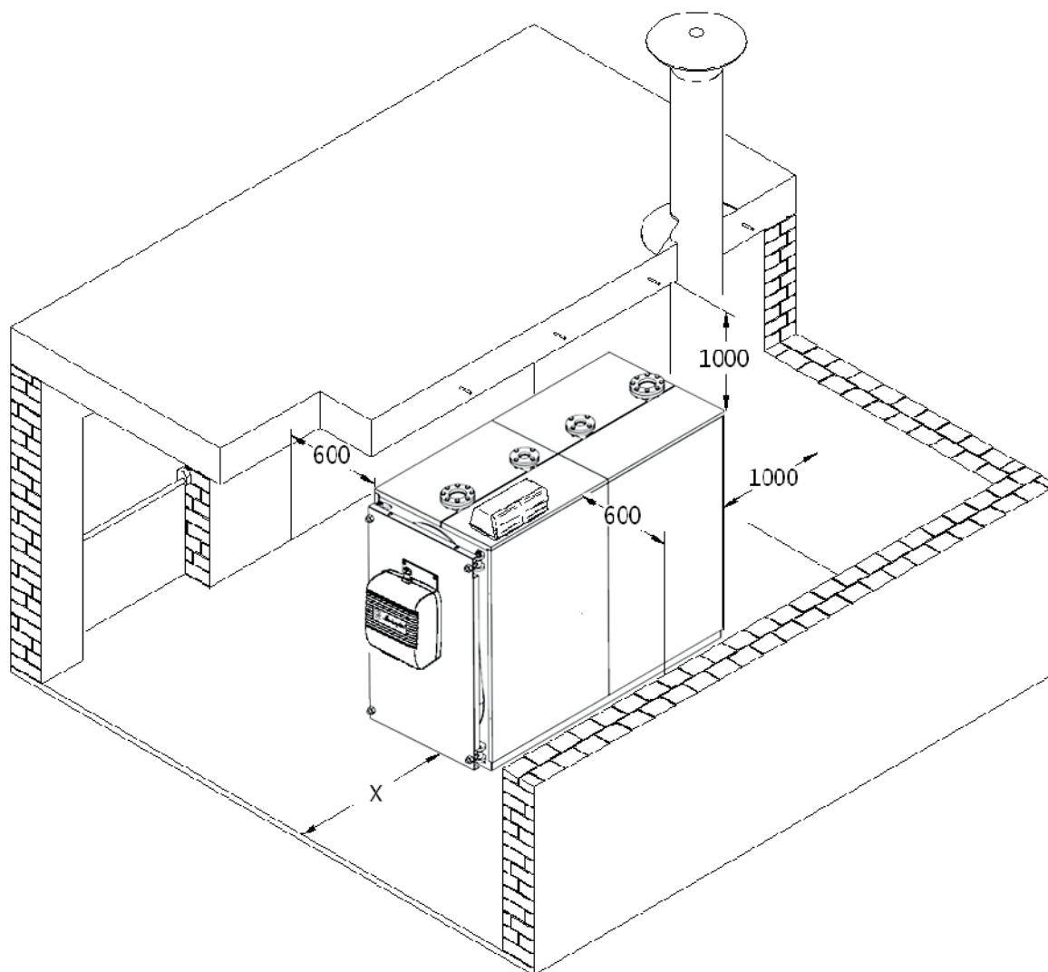
Fig. 6 - Installation room
