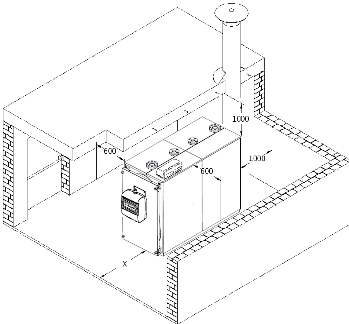
Fig. 4 - Installation room
