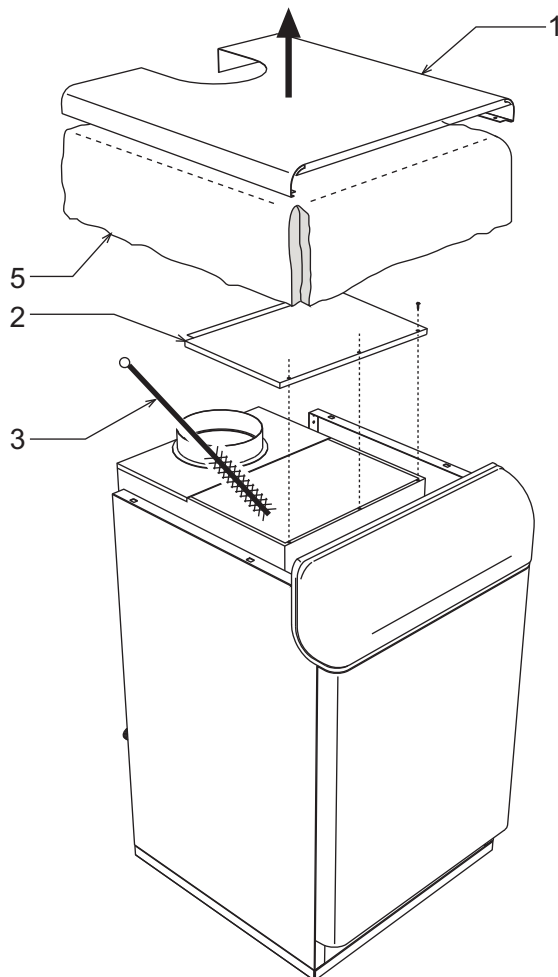
fig. 50 - Cleaning the boiler
