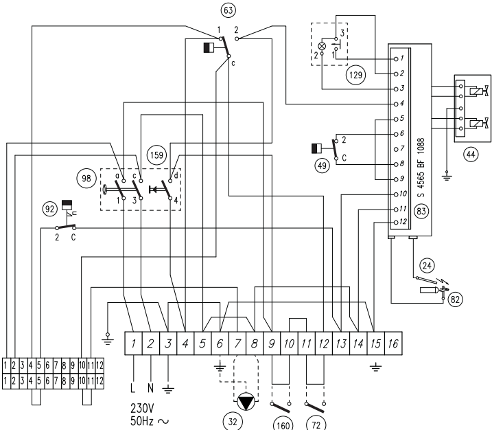
fig. 60 - Electrical connection diagram
