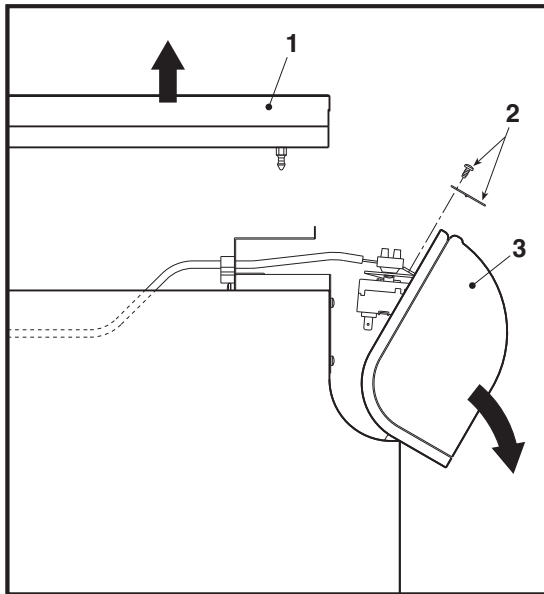
fig. 47 - Control panel opening
