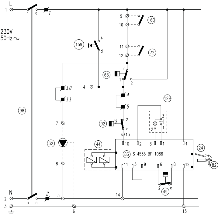
fig. 59 - Main wiring diagram
