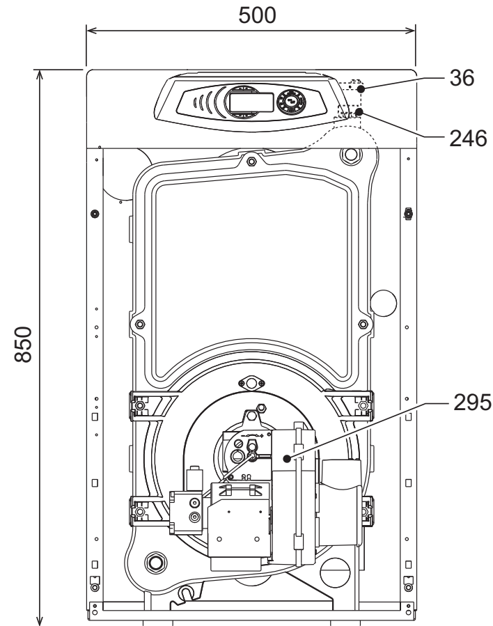
fig. 33 - Dimensions, connections and main components
