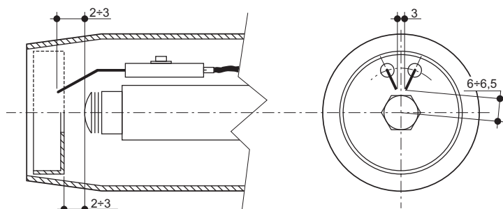
fig. 28- Position of electrodes - baffle
