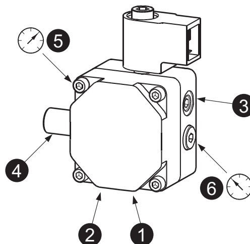
fig. 25- Pump DANFOSS
