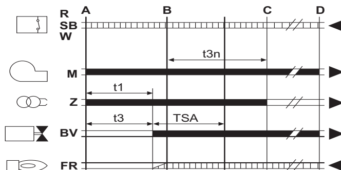
fig. 30 - Unit cycle
