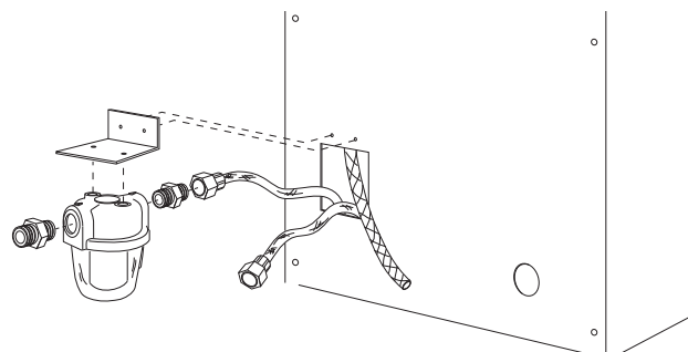
fig. 17 - Fuel filter installation
