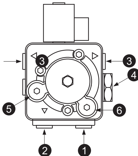
fig. 24- Pump ITALPUMP
