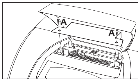
fig. 22 - Accessing the terminal board
