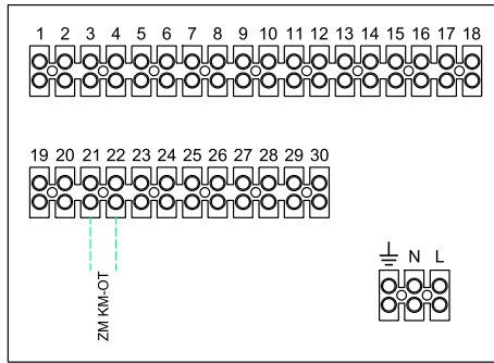
GENERATOR TERMINAL BLOCK
