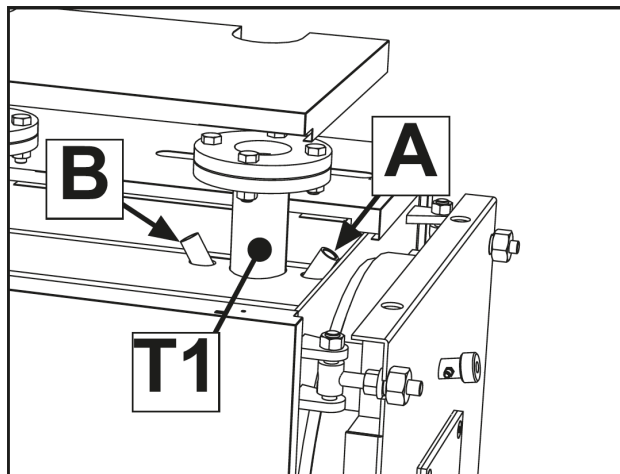
fig. 15 - Probe and bulb wells
