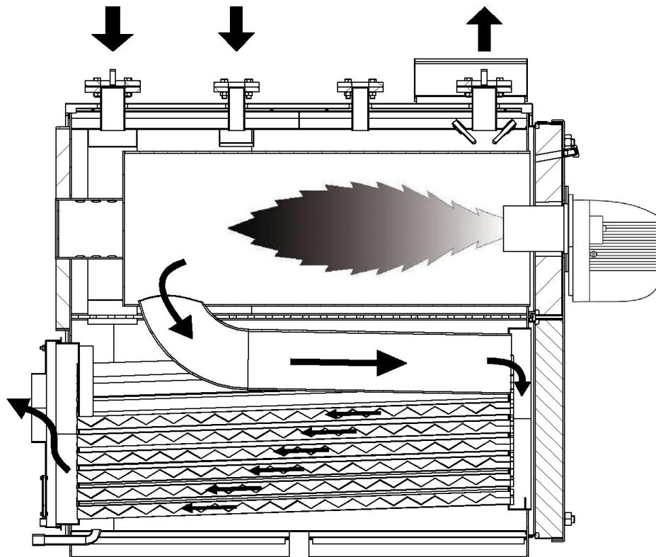
fig. 1 - Working principle
