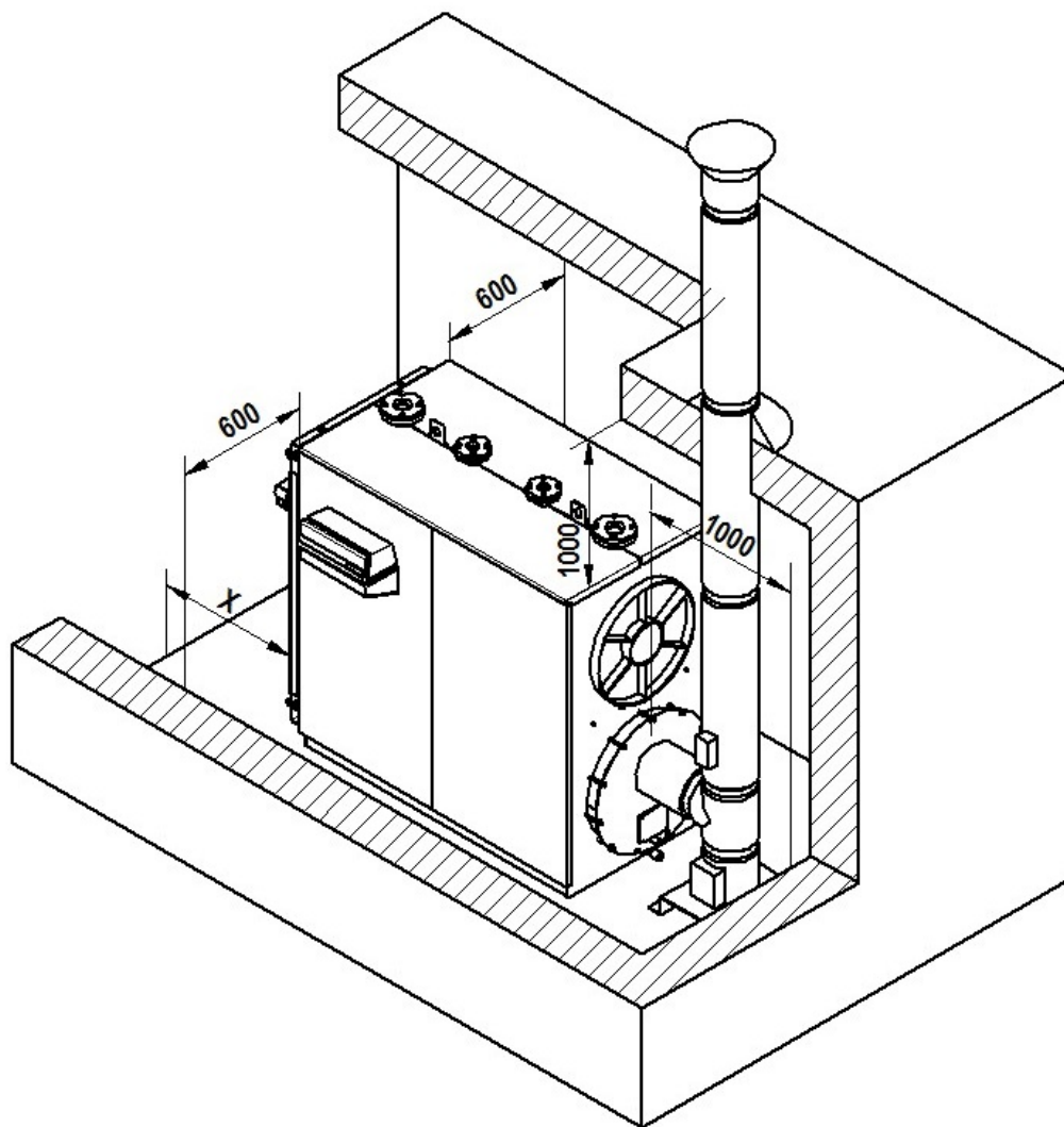
fig. 6 - Installation room
