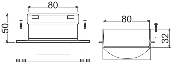
fig. 32 - Starting accessory for separate ducts
