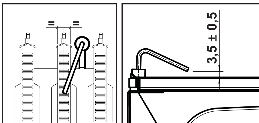
fig. 40- Electrode positioning
