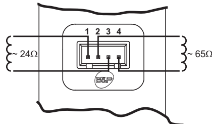
fig. 38 - Gas valve connection
