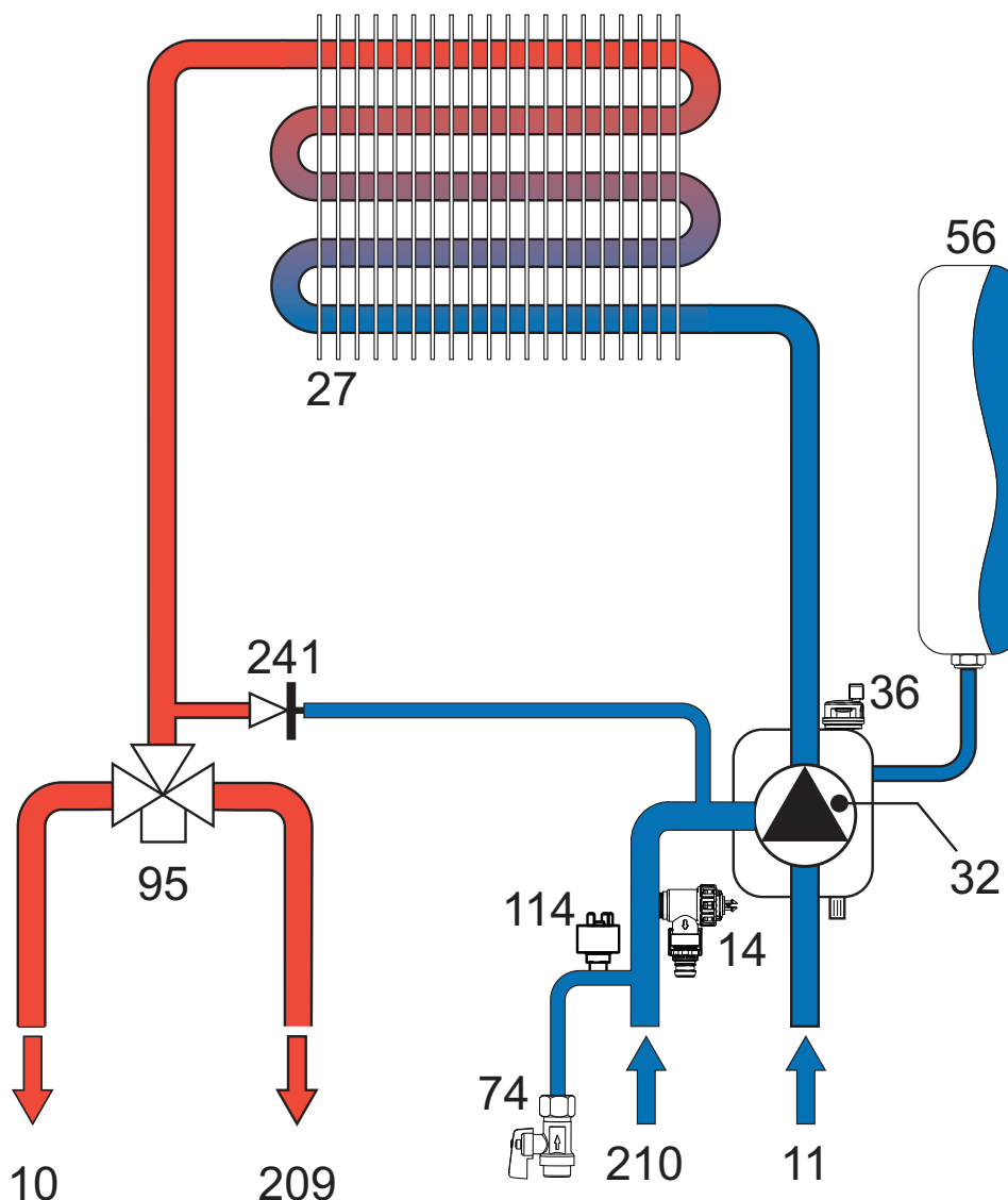
fig. 45- Heating circuit
