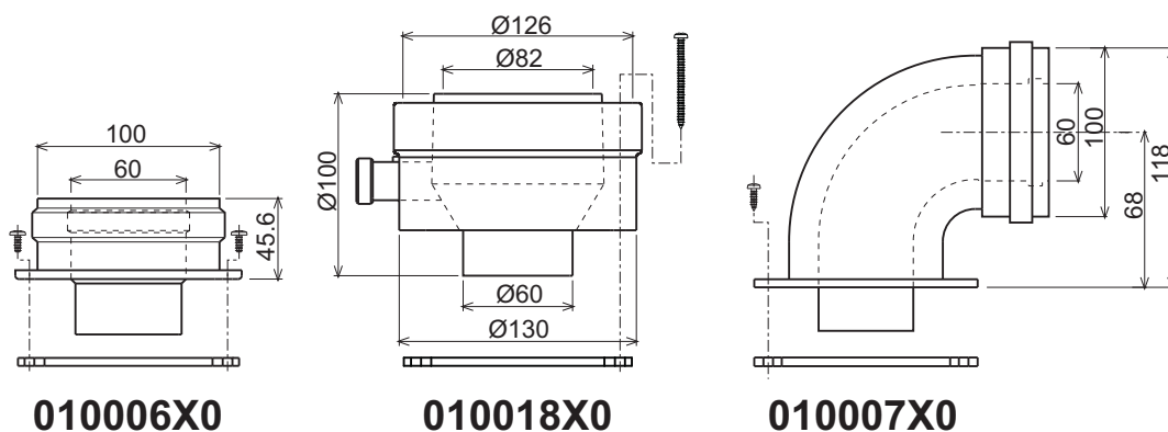
fig. 30- Starting accessories for coaxial ducts
