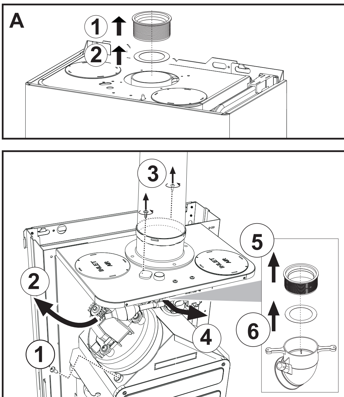
fig. 28- Baffle replacement
