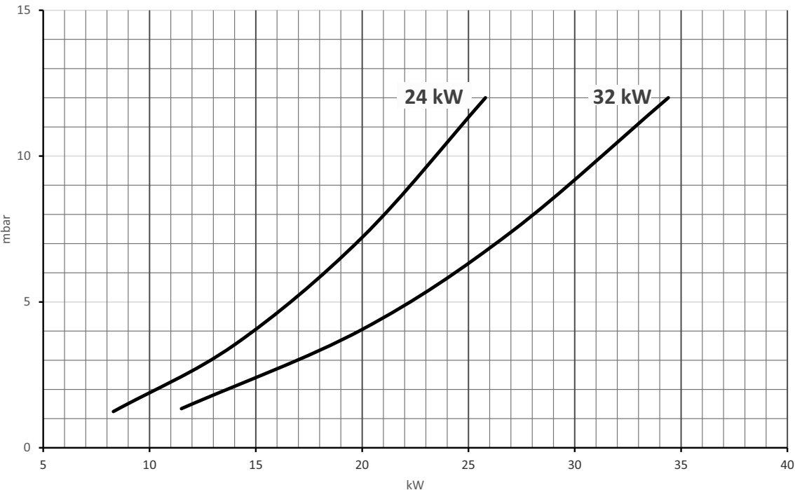
fig. 46- Diagram for Natural Gas versions
