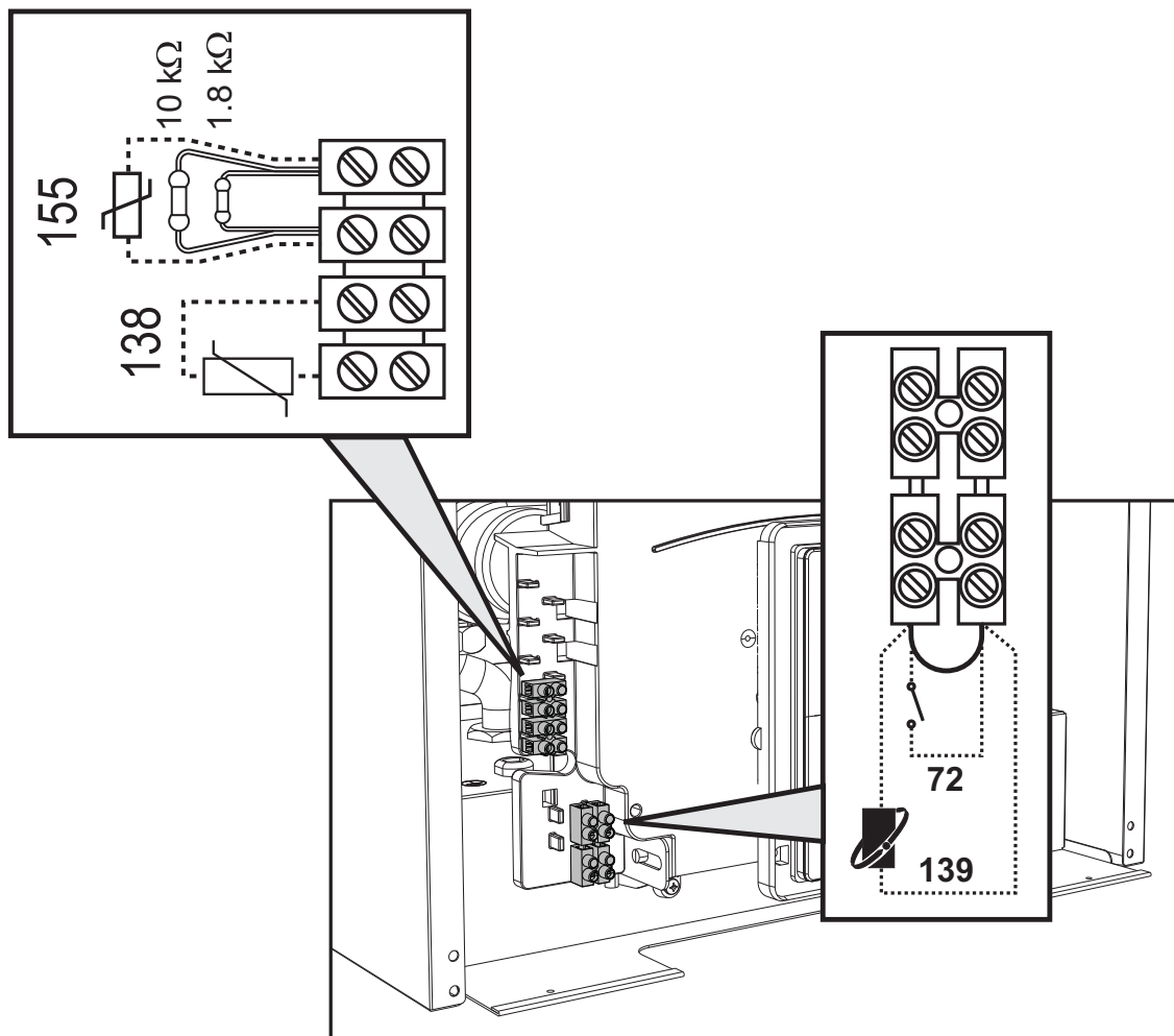
fig. 27- Accessing the terminal block
