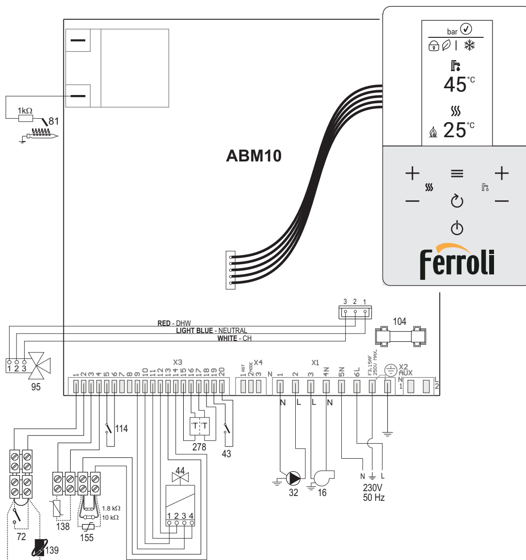
fig. 48- Wiring diagram
