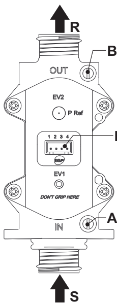
fig. 37 - Gas valve
