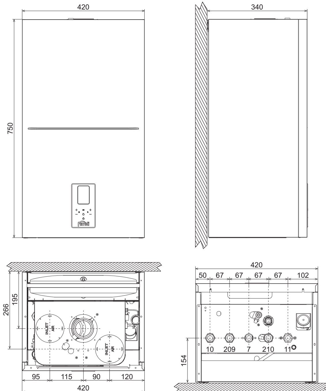
fig. 41- Dimensions and connections model DIVATOP D HF24
