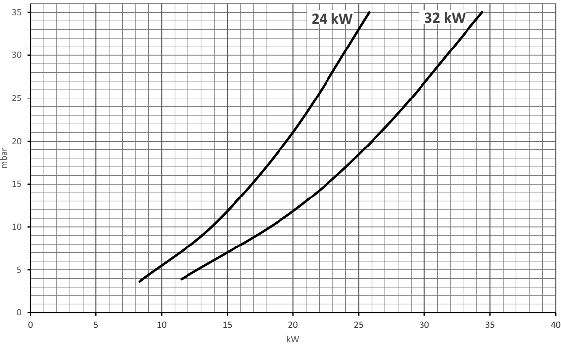
fig. 47- Diagram for LPG versions
