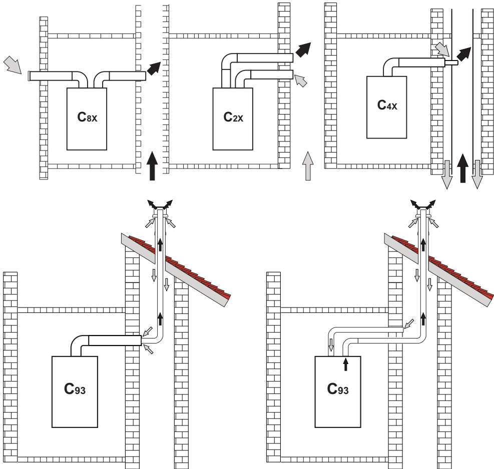
fig. 33 - Examples of connection to collective flues (⇐ = Air / ➡ = Fumes)
