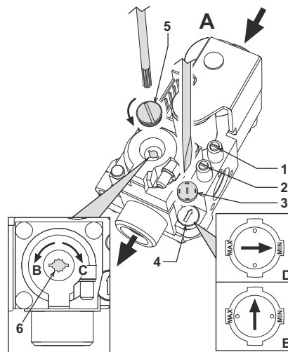
fig. 17 - Pressure adjustment
