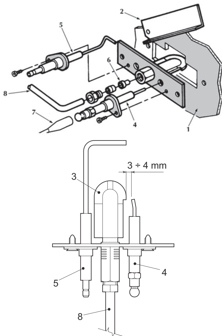
fig. 21 - Pilot burner
