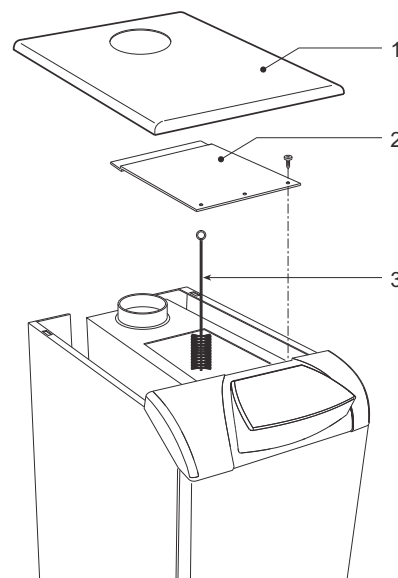
fig. 19 - Boiler cleaning
