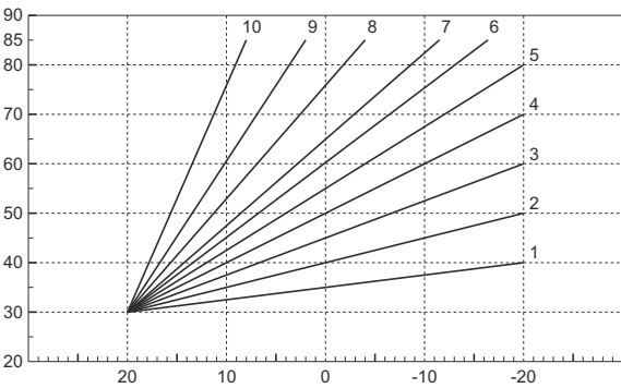
fig. 11 - Compensation curves
