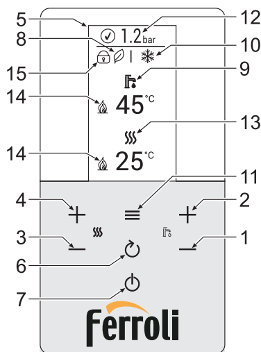
fig. 1 - Control panel
