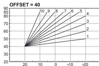
fig. 25 - Example of compensation parallel curve offset
