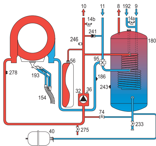
fig. 45 - Hydraulic circuit
