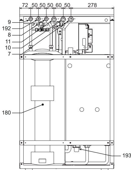
fig. 43 - Rear View
