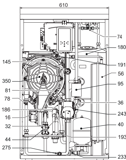
fig. 41 - Front view
