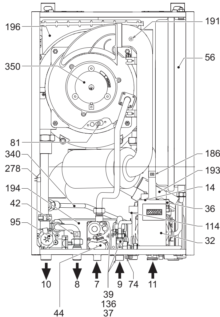
fig. 26 - General view
