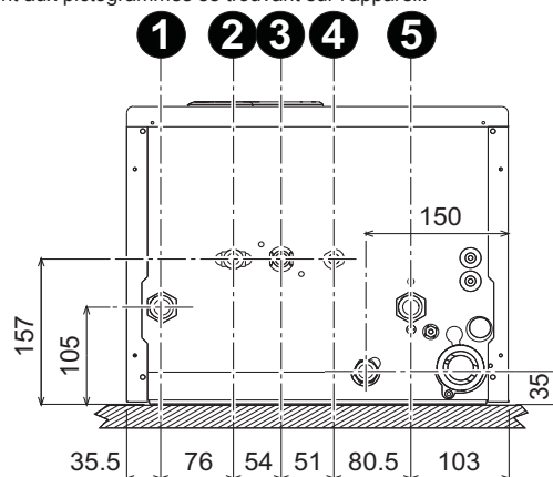
fig. 13 - Raccordements hydrauliques
