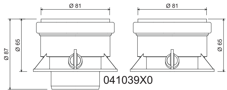
fig. 18 - Starting accessory for separate ducts
