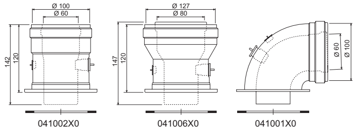
fig. 16 - Starting accessory for coaxial ducts
