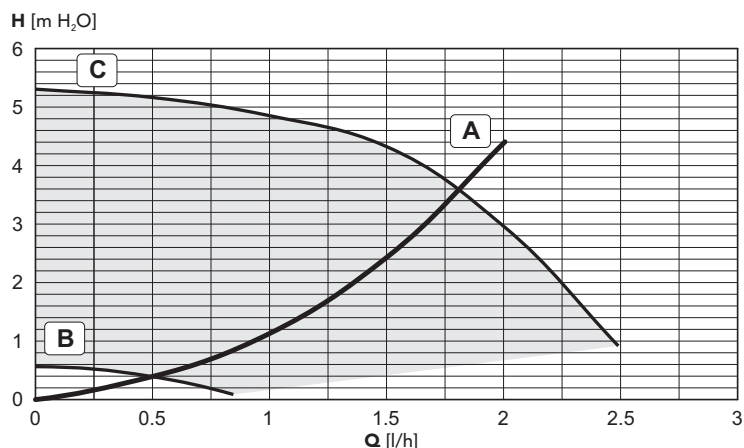
fig. 28 - Circulating pump head / Pressure losses BLUEHELIX TECH 25 C
