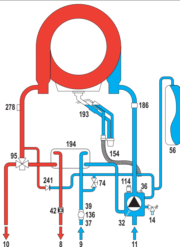
fig. 27 - Water circuit
