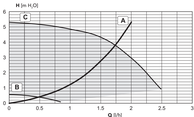
fig. 29 - Circulating pump head / Pressure losses BLUEHELIX TECH 35 C
