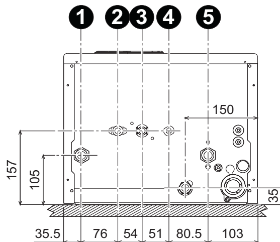
fig. 13 - Plumbing connections
