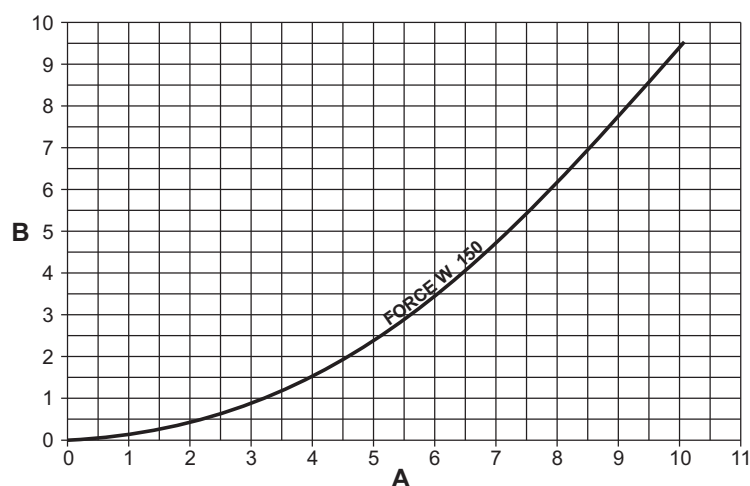
fig. 85- Pressure loss diagram - models FORCE W 150
