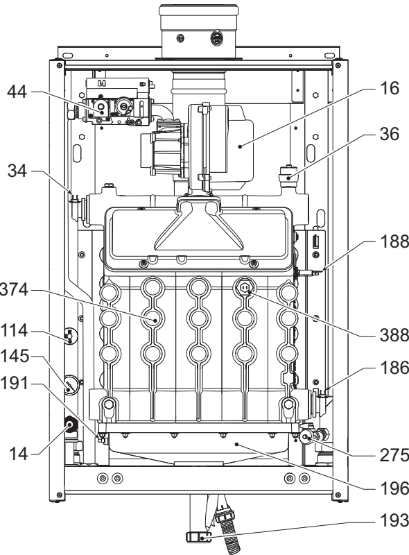
fig. 82- Vista general mod. FORCE W 150
