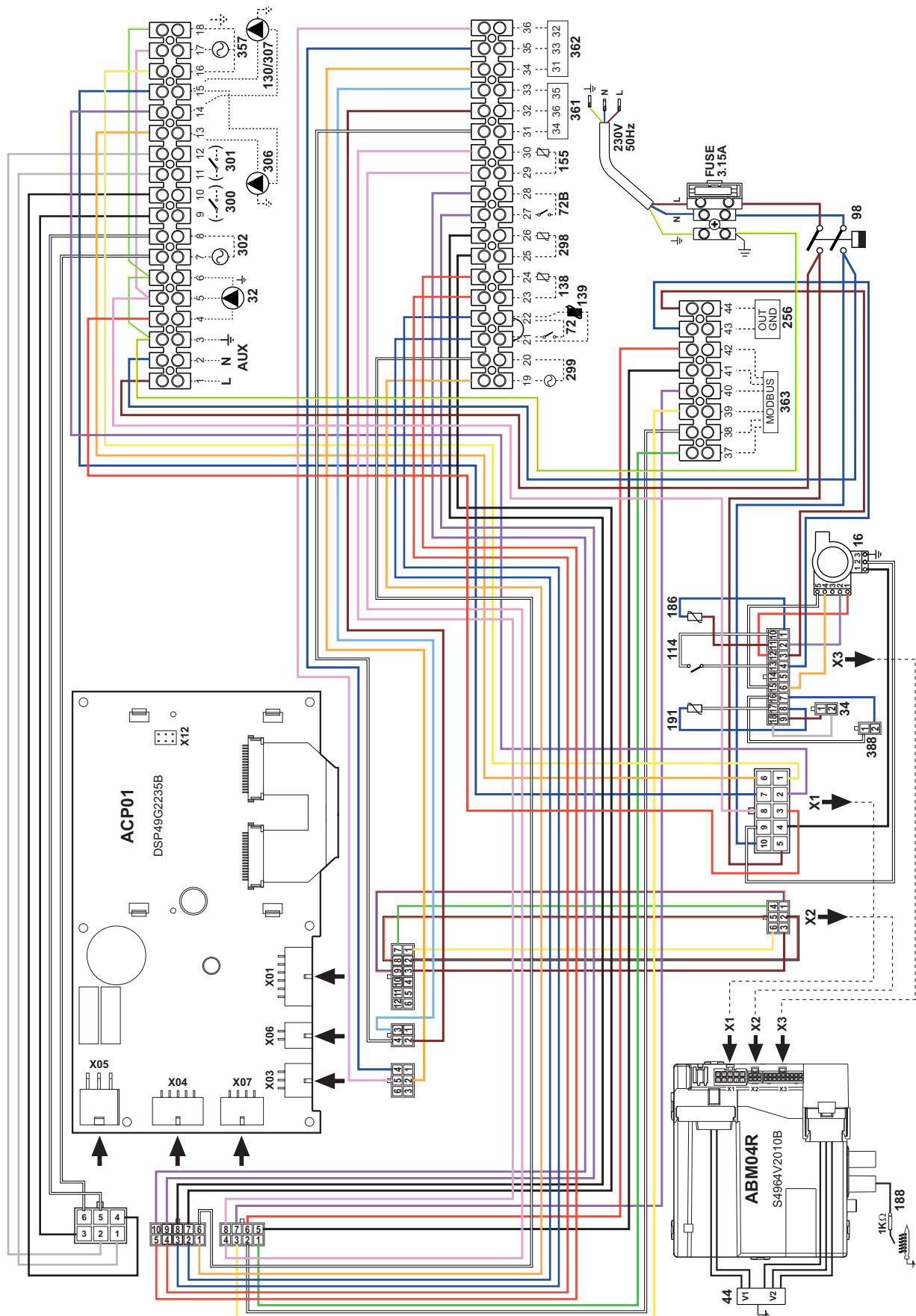
fig. 90- Wiring diagram - models FORCE W 99, FORCE W 120 and FORCE W 150
