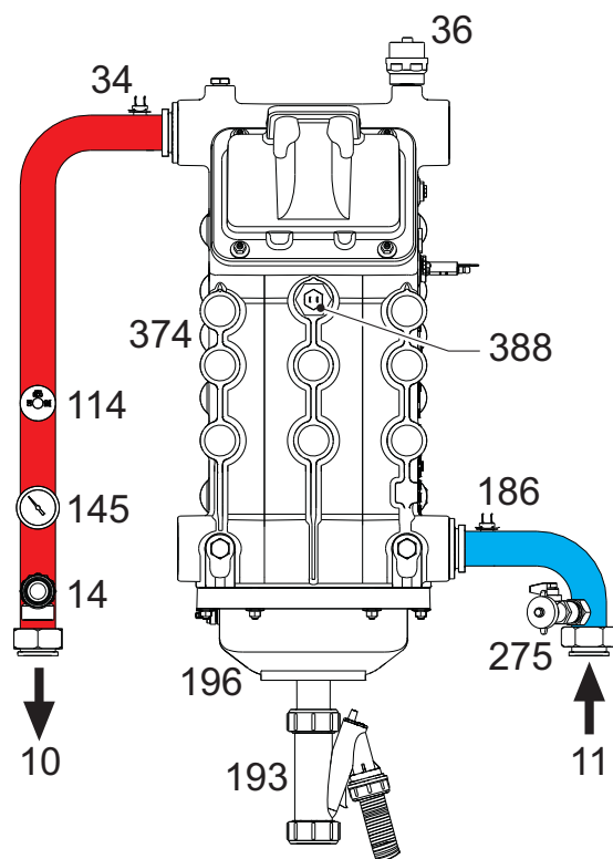
fig. 83- Hydraulic circuit
