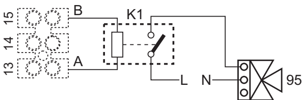
fig. 86- Connection of the 3-way valve with 2 wires
