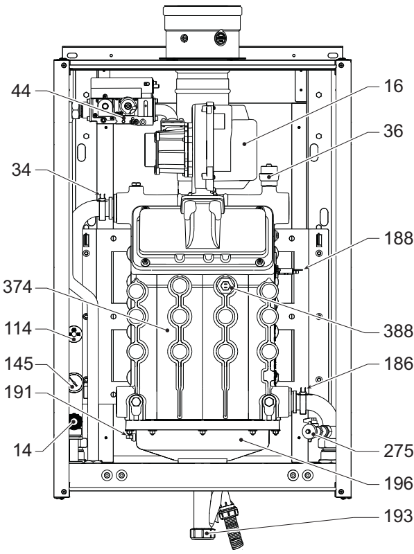
fig. 81- General view - model FORCE W 99 and FORCE W 120
