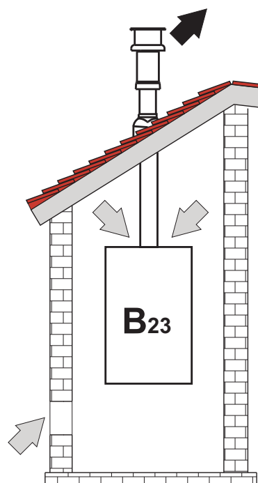
fig. 58- Connection examples (⇨=Air / ⇨=Fumes)
