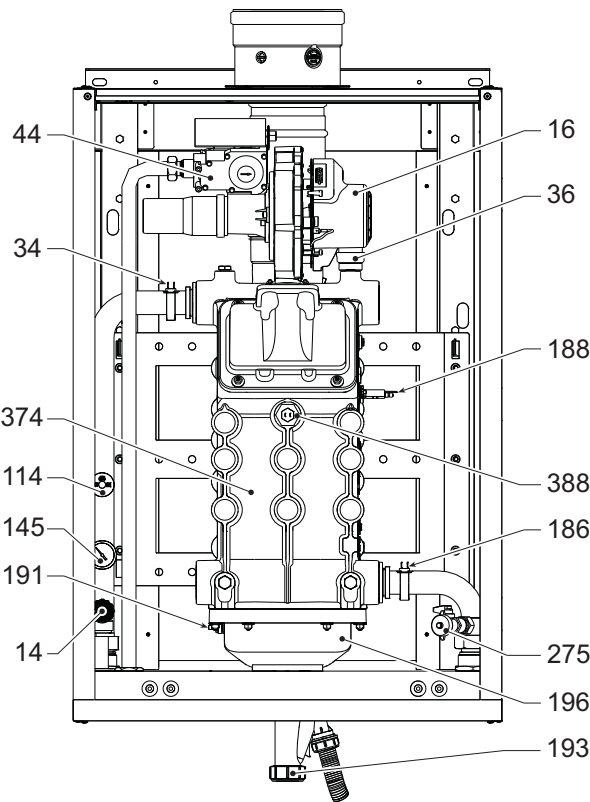
fig. 80- Vista general mods. FORCE W 60 y FORCE W 80
