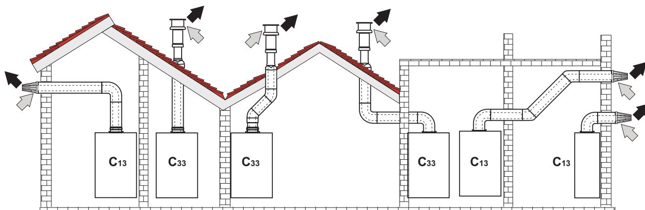
fig. 59- Examples of connection with coaxial pipes (→ = Air / → = Fumes)
