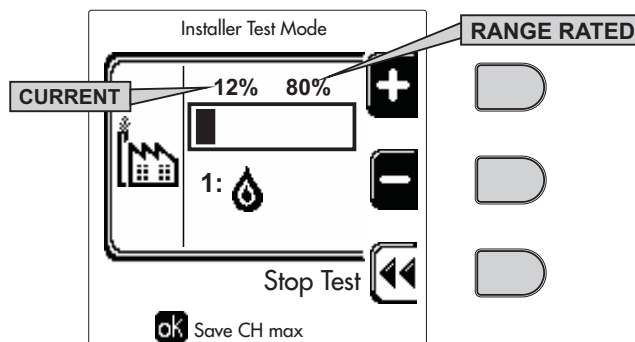
fig. 73- TEST mode (ex. heating power = 80%)
