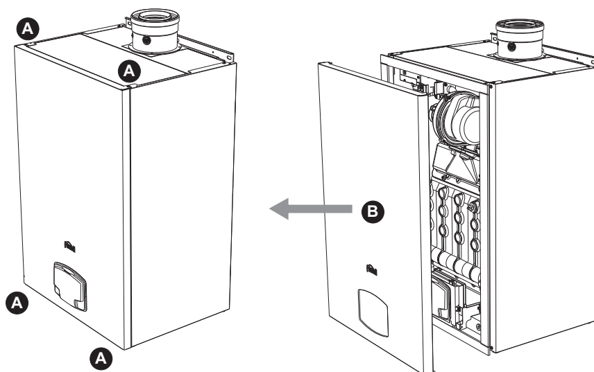
fig. 75- Front panel opening
