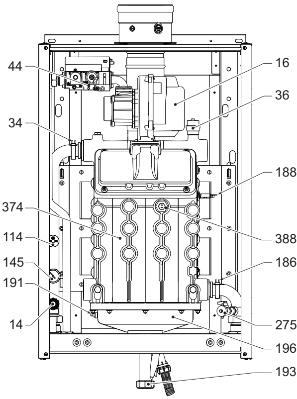
fig. 81- Vista general mods. FORCE W 99 y FORCE W 120
