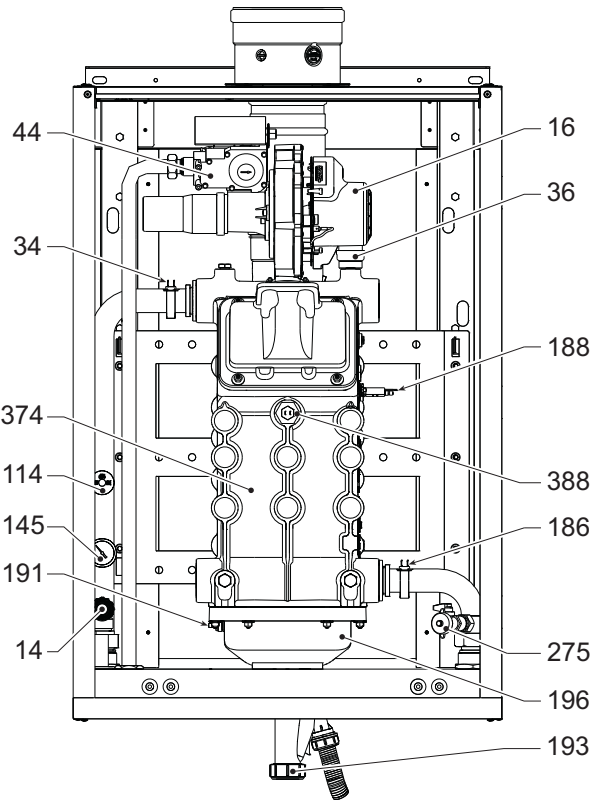
fig. 80- General view - model FORCE W 60 and FORCE W 80
