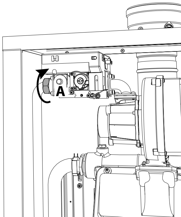
fig. 62- Models W 99, W 120 and W 150
