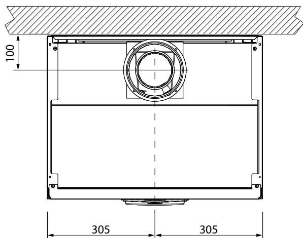
fig. 78- Top view
