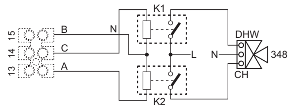
fig. 87- Connection of the 3-way valve with 3 wires
