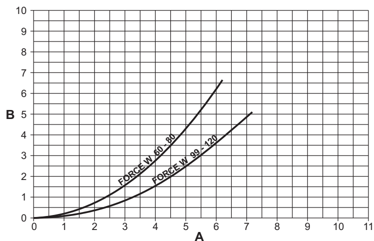
fig. 84- Pressure loss diagram - models FORCE W 60 - FORCE W 80 - FORCE W 99 - FORCE W 120
