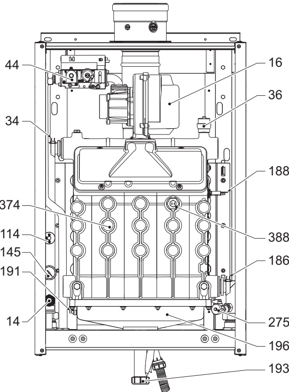
fig. 82- General view - model FORCE W 150
