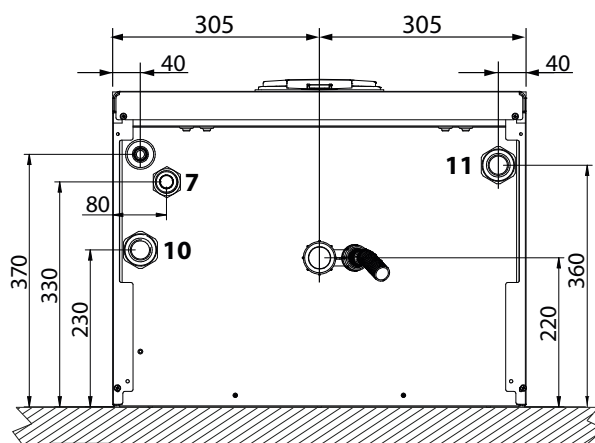
fig. 79- Bottom view
