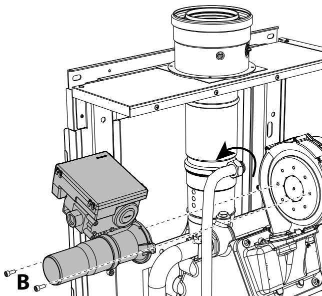
fig. 63- Models W 60 and W 80
