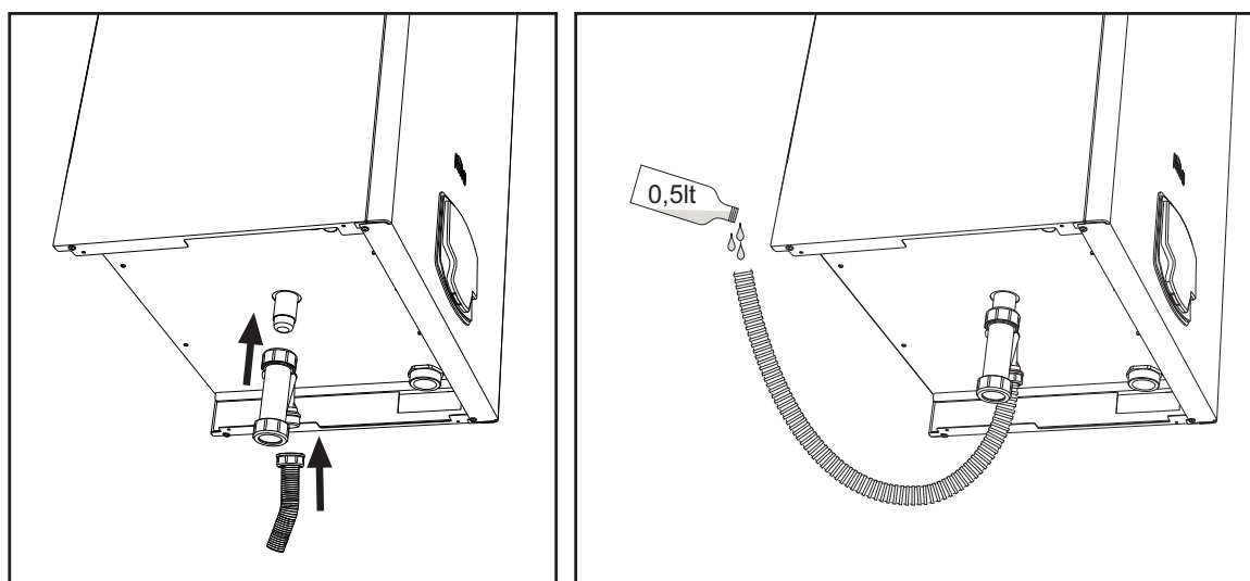
fig. 60- Condensate drain connection
