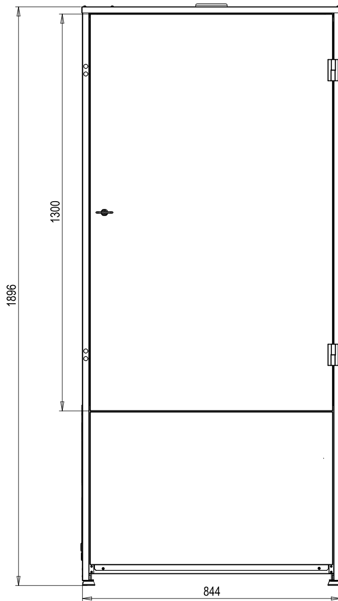
Vista frontal
